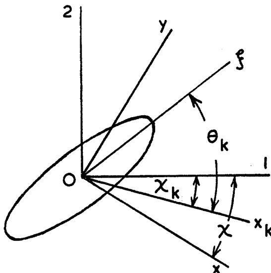
FIG. 9. Parameters for a polydisperse system (Sadron). Ox and Oy are the principal vibration directions of the solution, Ox_k is the direction of preferred orientation of type k particles, and O1 is the flow direction.
