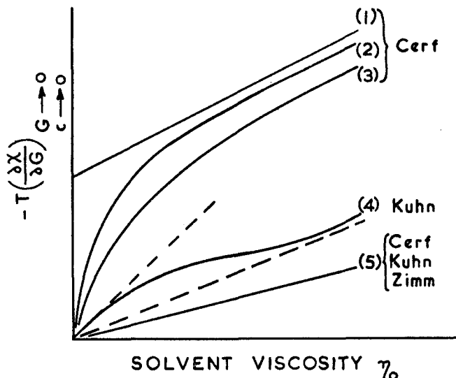
FIG. 22. Variation of T(-\delta\chi/\delta G)_{G \rightarrow 0, c \rightarrow 0} with solvent viscosity for different theories at very small concentration. Curve (1), elastic sphere model, \delta_o = 0 , equations 189, 192; Rouse model, equation 196. Curve (2), elastic sphere model, \delta_o = 0.1 , equation 187. Curve (3), elastic sphere model, \delta_o = 0.2 , equation 187. Curve (4), elastic dumbbell model: the curve lies between the dotted lines which are the curves given by equation 155 for stiff and soft molecules. Curve (5), rigid particle (Cerf, equations 190 and 197; Kuhn, equation 192, Zimm, equation 202).
