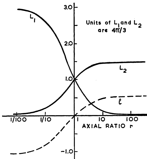
FIG. 11. Shape factors L_1 and L_2 (or L_\xi and L_\eta ) as functions of axial ratio r . These factors are given by L_1 = \frac{4\pi}{3} (1 - 2l) and L_2 = \frac{4\pi}{3} (1 + l) , and the variation of l with r is also shown (see Appendix 2).
